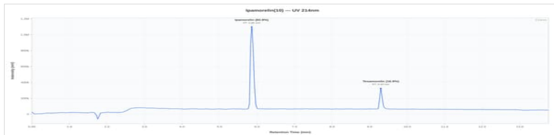
CJC-1295 (No DAC)/ Ipamorelin 10mg - LOT-2026-001: UV Chromatogram
