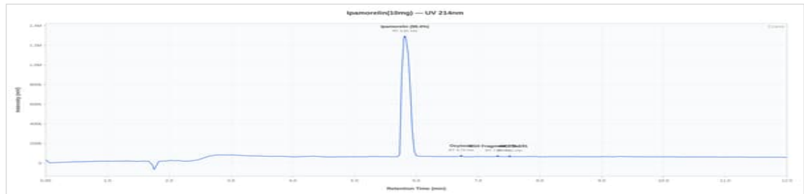
Ipamorelin 10mg - LOT-2026-001: UV Chromatogram
